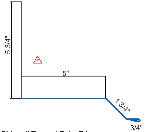
Sidewall/Parapet Rake Trim
